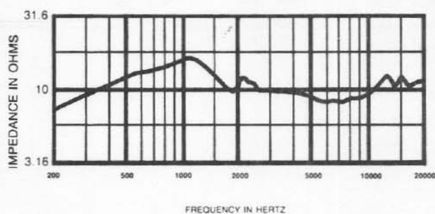
FIGURE 7 Impedance Response — HP9040 Horn
