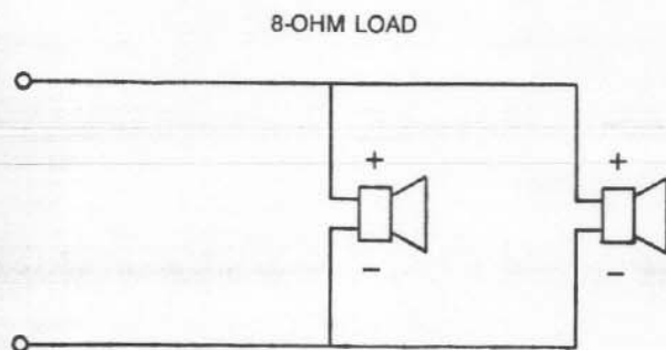
FIGURE 8 Electrical Connections
