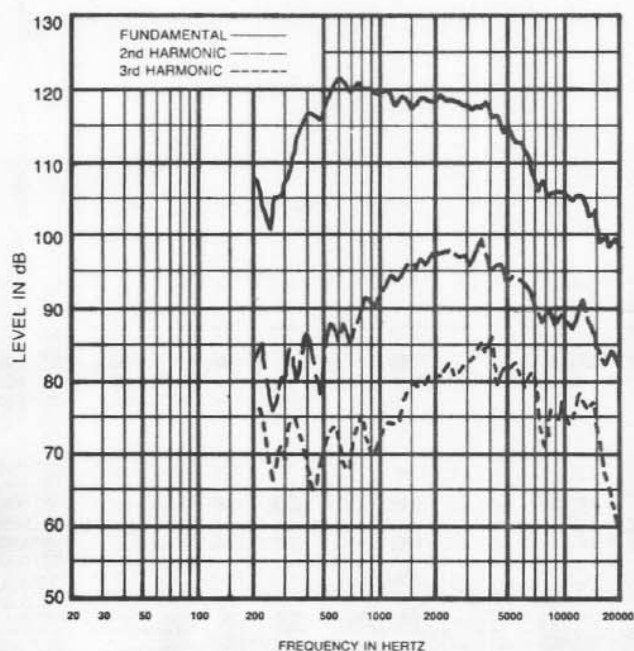
FIGURE 5 Distortion Response, HP9040 Horn, 10 Watts/1 Meter
